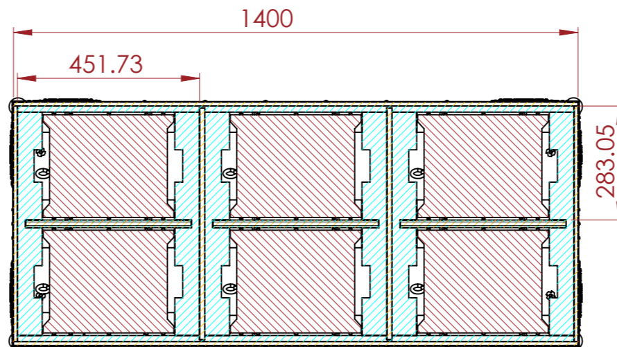
SECTION C-C
