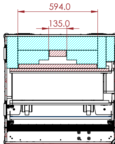
SECTION C-C
