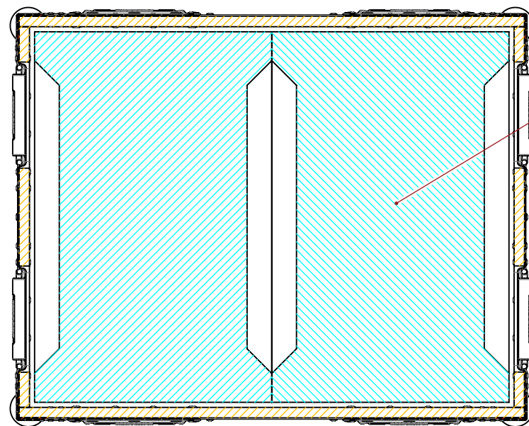
SECTION B-B SCALE 1 : 6.5
