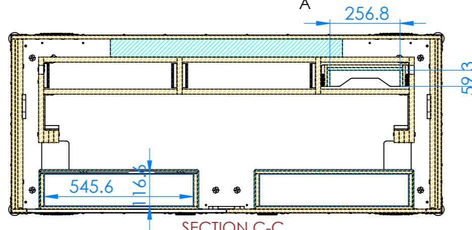
SECTION C-C
