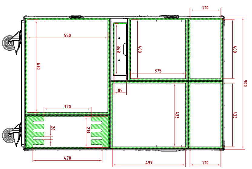
LEFT BODY CASE
