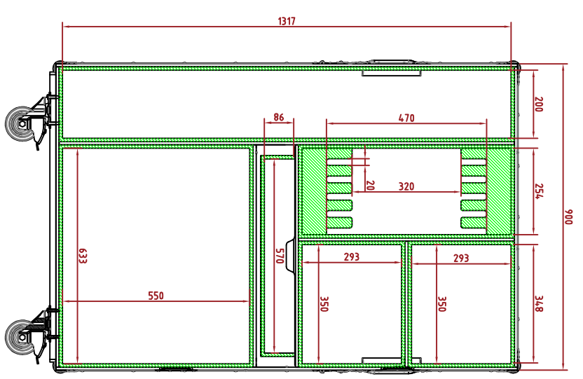
RIGHT BODY CASE
