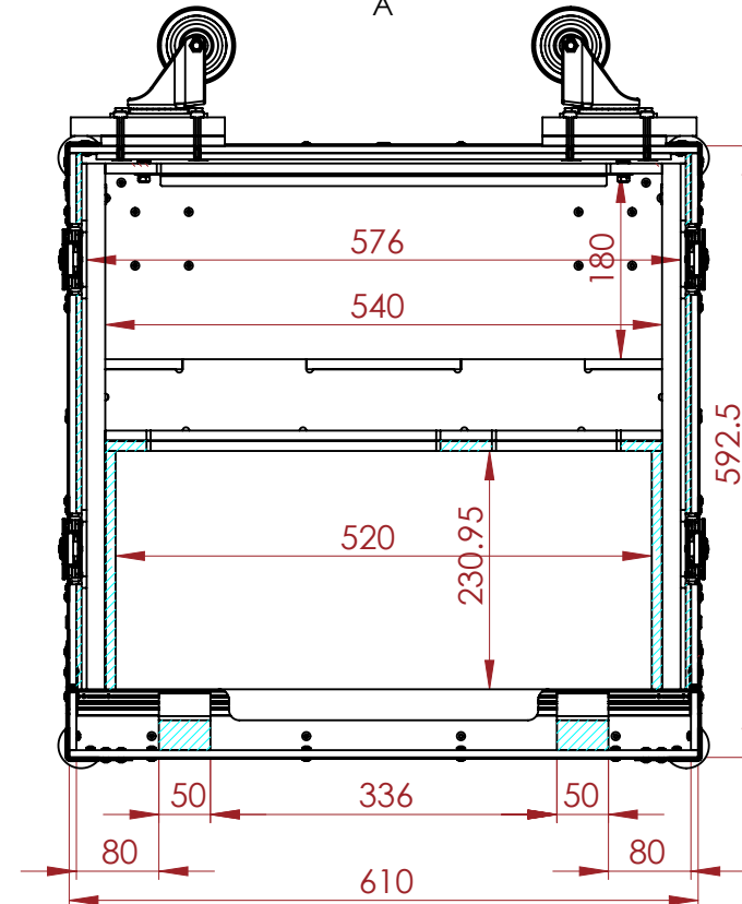
SECTION C-C
