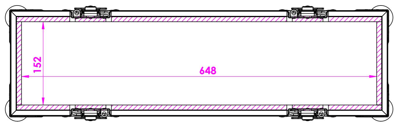
Top Cutout View
