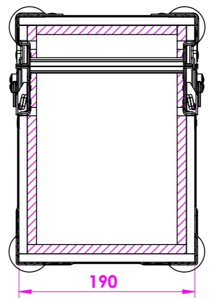
Side Cutout View
