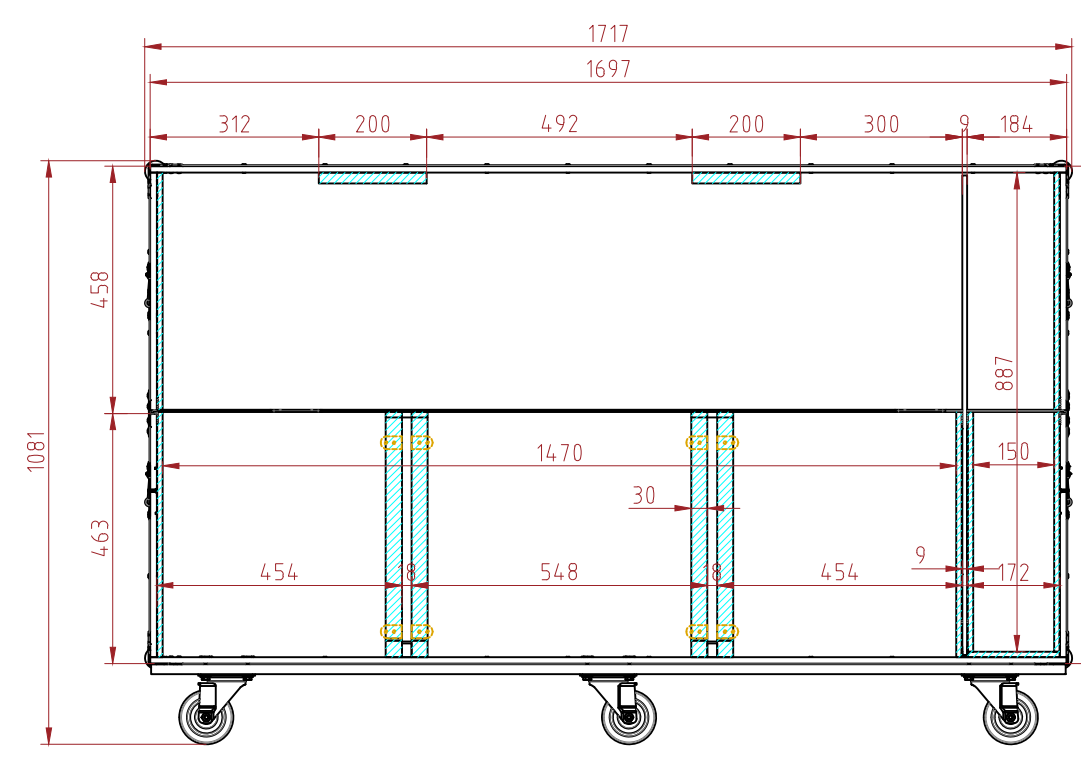
FRONT VIEW
